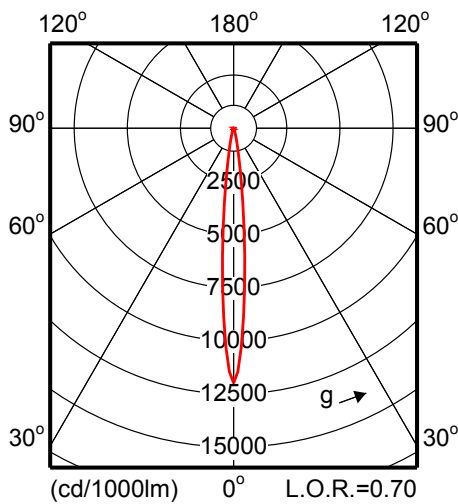
MRS561 1xCDM-T35W EB 12
