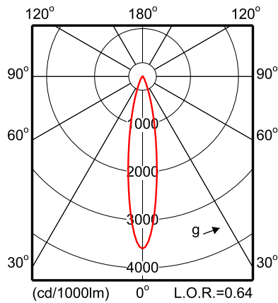
MCS561 1xCDM-T70W EB 24-36 P24
