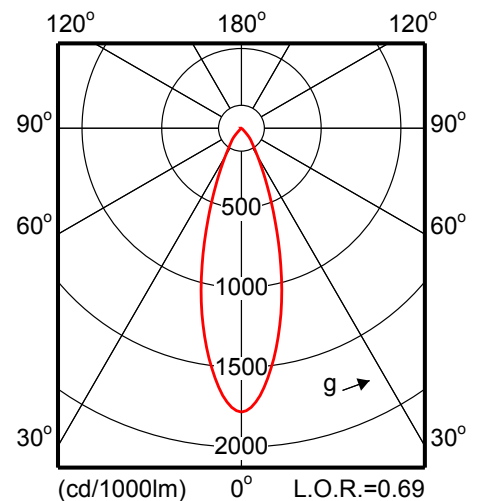
MCS561 1x CDM-T70W EB 24-36 P36
