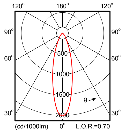
MRS561 1xCDM-T150W EB 36
