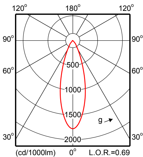
MRS561 1x CDM-T70W EB 24-36 P36
