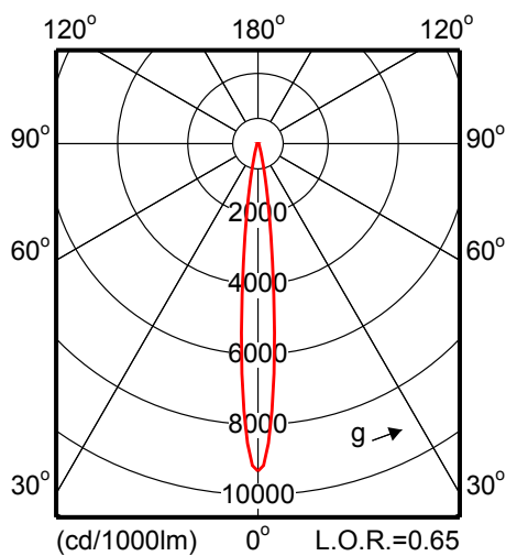
MRS561 1xCDM-T70W EB 12-24 P12
