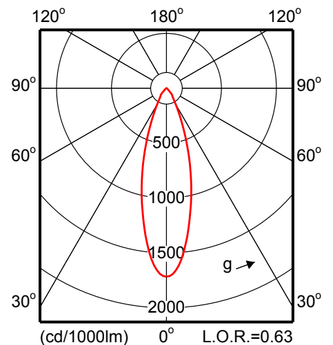
MRS561 1xCDM-T70W EB 36-CH
