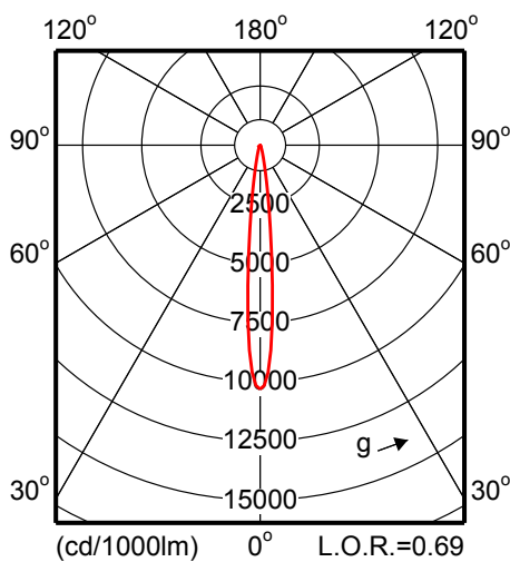
MRS561 1xCDM-T70W EB 12
