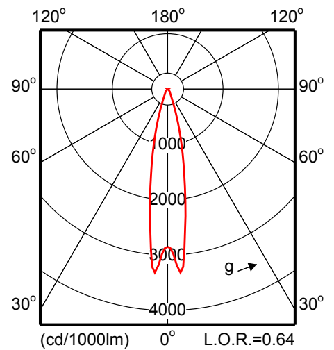
MRS561 1xCDM-T35W EB 12-24 P24
