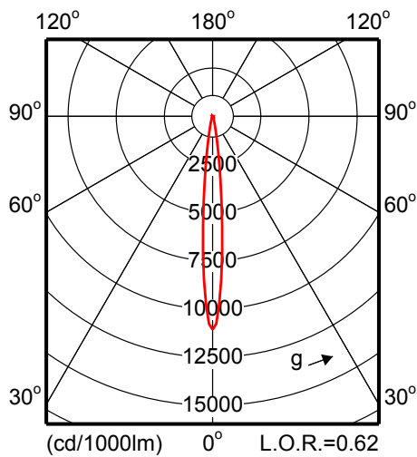
MRS561 1xCDM-T35W EB 12-24 P12
