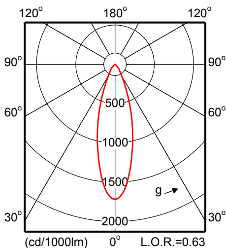
MCS561 1xCDM-T70W EB 36-CH
