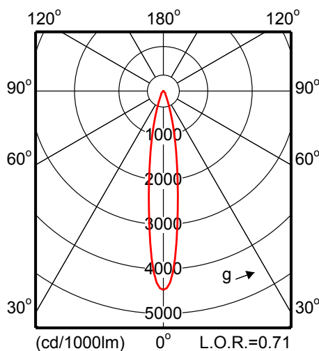
MCS561 1xCDM-T70W EB 24
