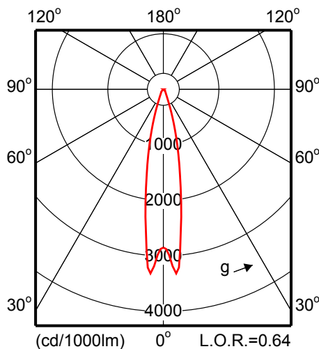
MRS561 1xCDM-T35W EB 12-24 P24
