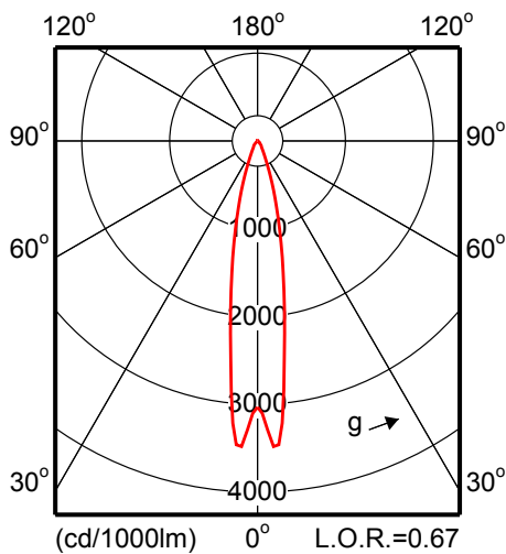
MRS561 1xCDM-T70W EB 12-24 P24
