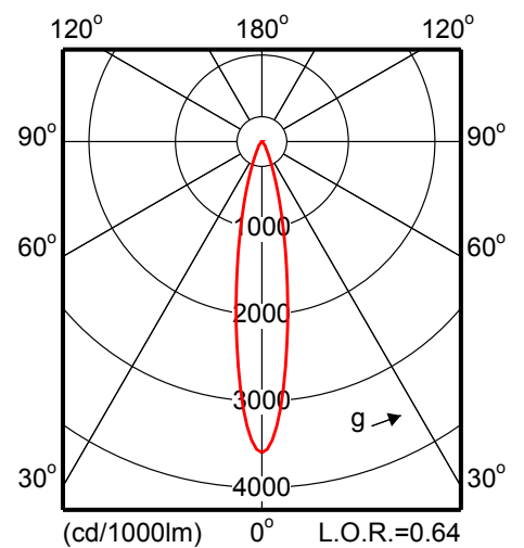
MRS561 1x CDM-T70W EB 24-36 P24
