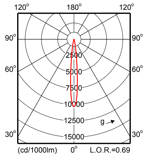
MRS561 1x CDM-T70W EB 12
