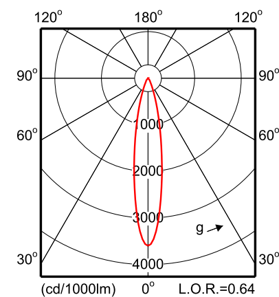
MRS561 1x CDM-T70W EB 12-24 P12
