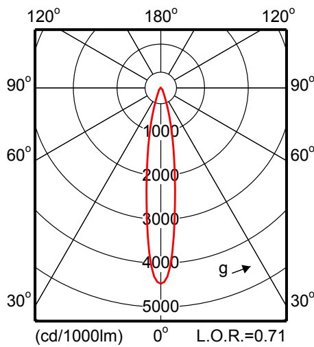
MRS561 1x CDM-T70W EB 24
