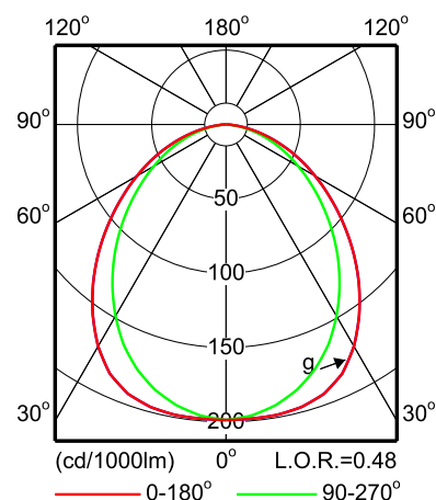
FBH024 2xPL-C/4P18W HF FRG
