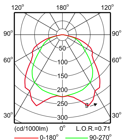
FBH024 2xPL-C/2P26W
