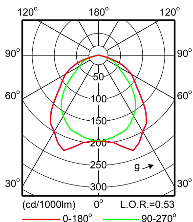
FBH024 2xPL-C/4P18W HF RG
