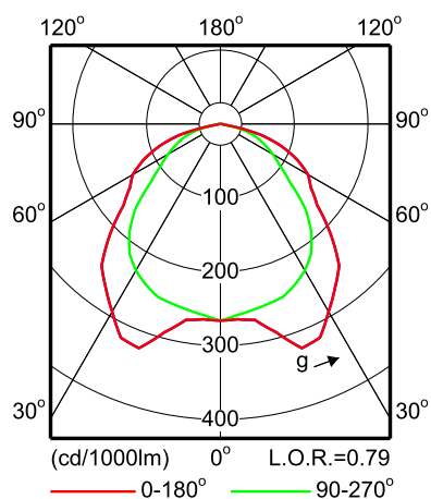
FBH024 2xPL-C/2P18W
