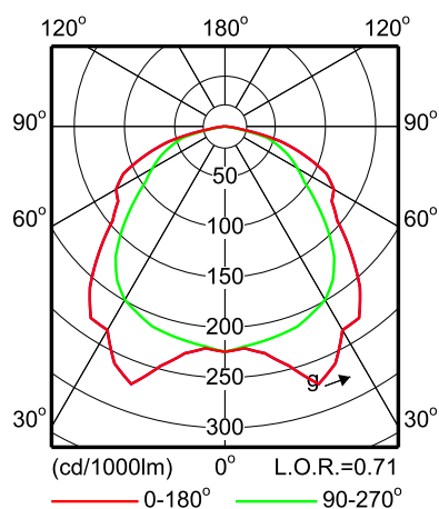
FBH024 2xPL-C/4P26W HF
