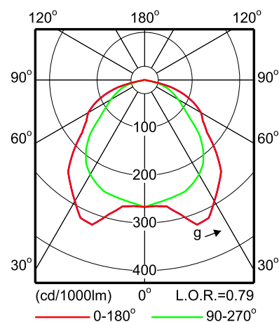
FBH024 2xPL-C/2P18W
