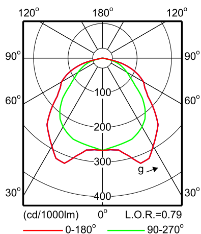
FBH024 2xPL-C/4P18W HF
