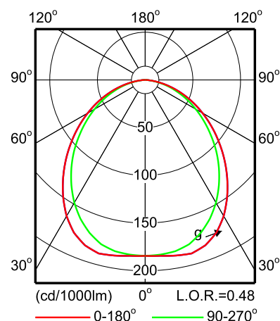
FBH024 2xPL-C/4P26W HF FRG
