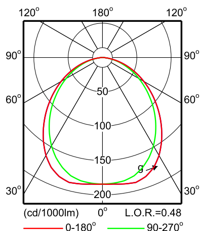
FBH024 2xPL-C/4P26W HF FRG
