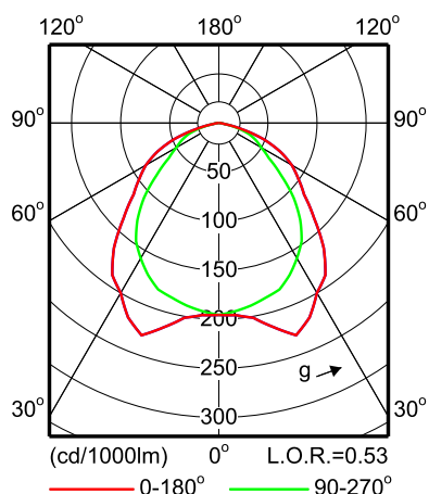
FBH024 2xPL-C/2P18W RG
