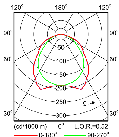
FBH024 2xPL-C/2P26W RG
