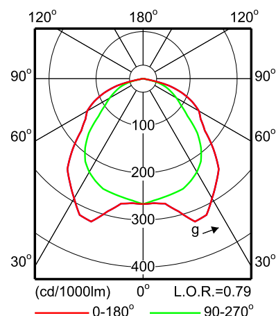
FBH024 2xPL-C/4P18W HF
