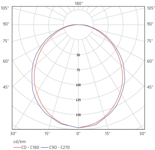
SATURN LED 9W
