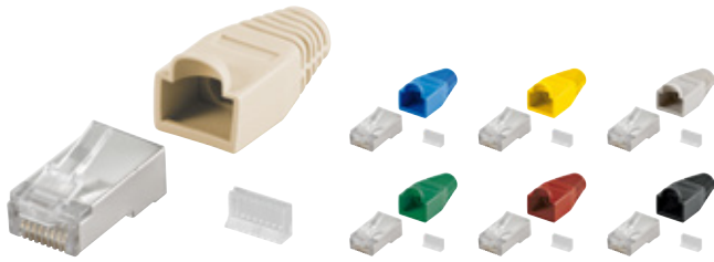
Goobay RJ45 plug, CAT 5e STP shielded with strain-relief boot for round cable with Threader
