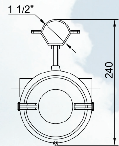
Mounting using 1.1/2" metal clamps TYPE "P"
